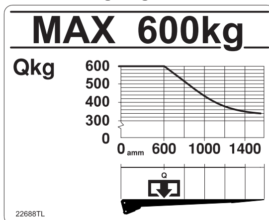
Loading diagram
